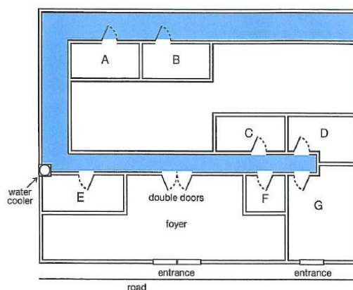
Ground floor plan of theatre
